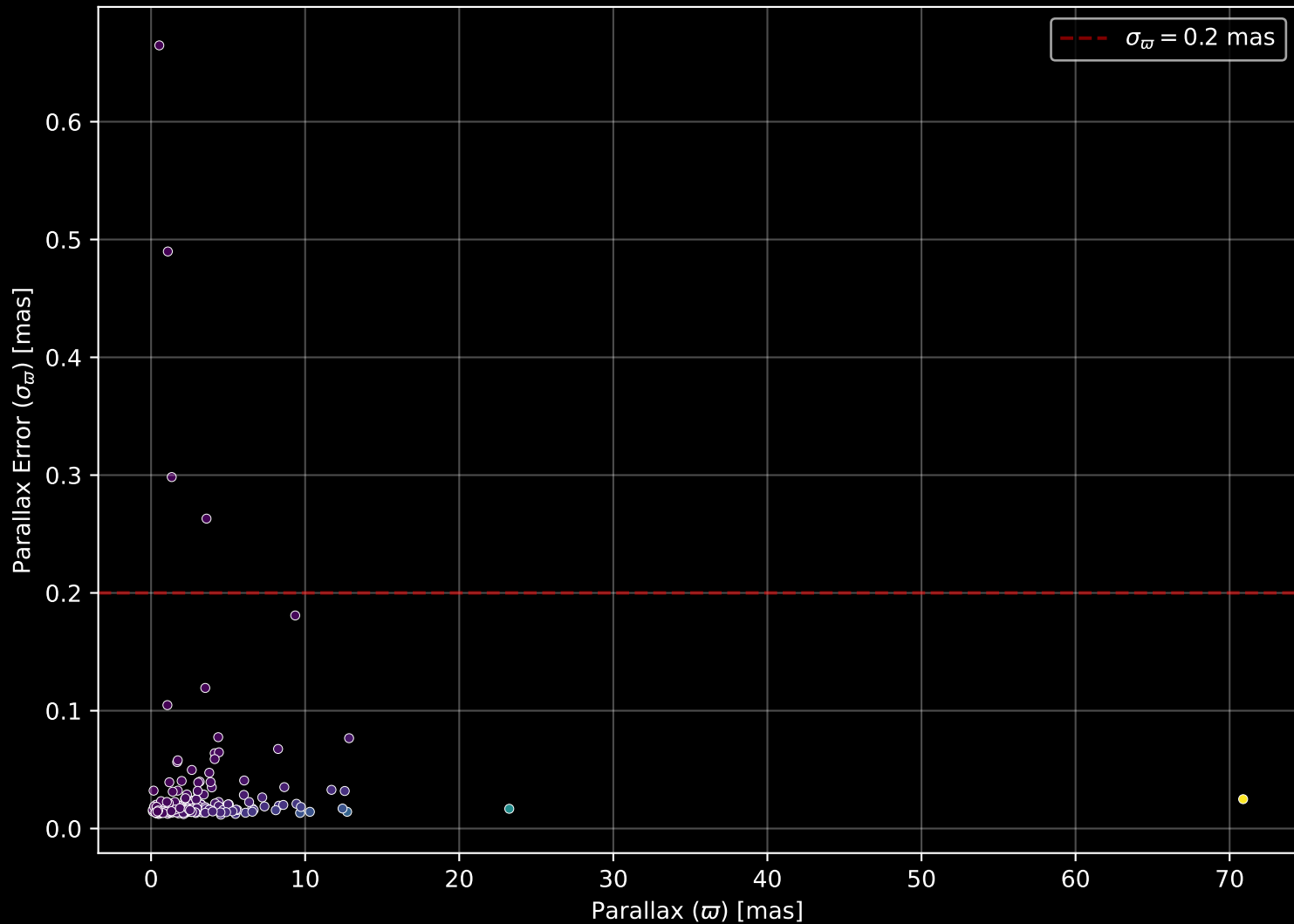
APOGEE DR17 Field: [168+30_MGA] Parallax Quality (n= 186)
