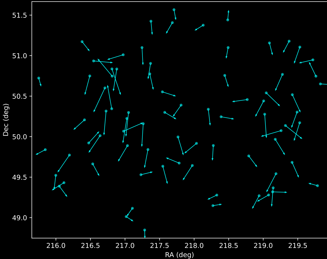
APOGEE DR17 Noise Stream Proper Motion Vectors (n=78)
