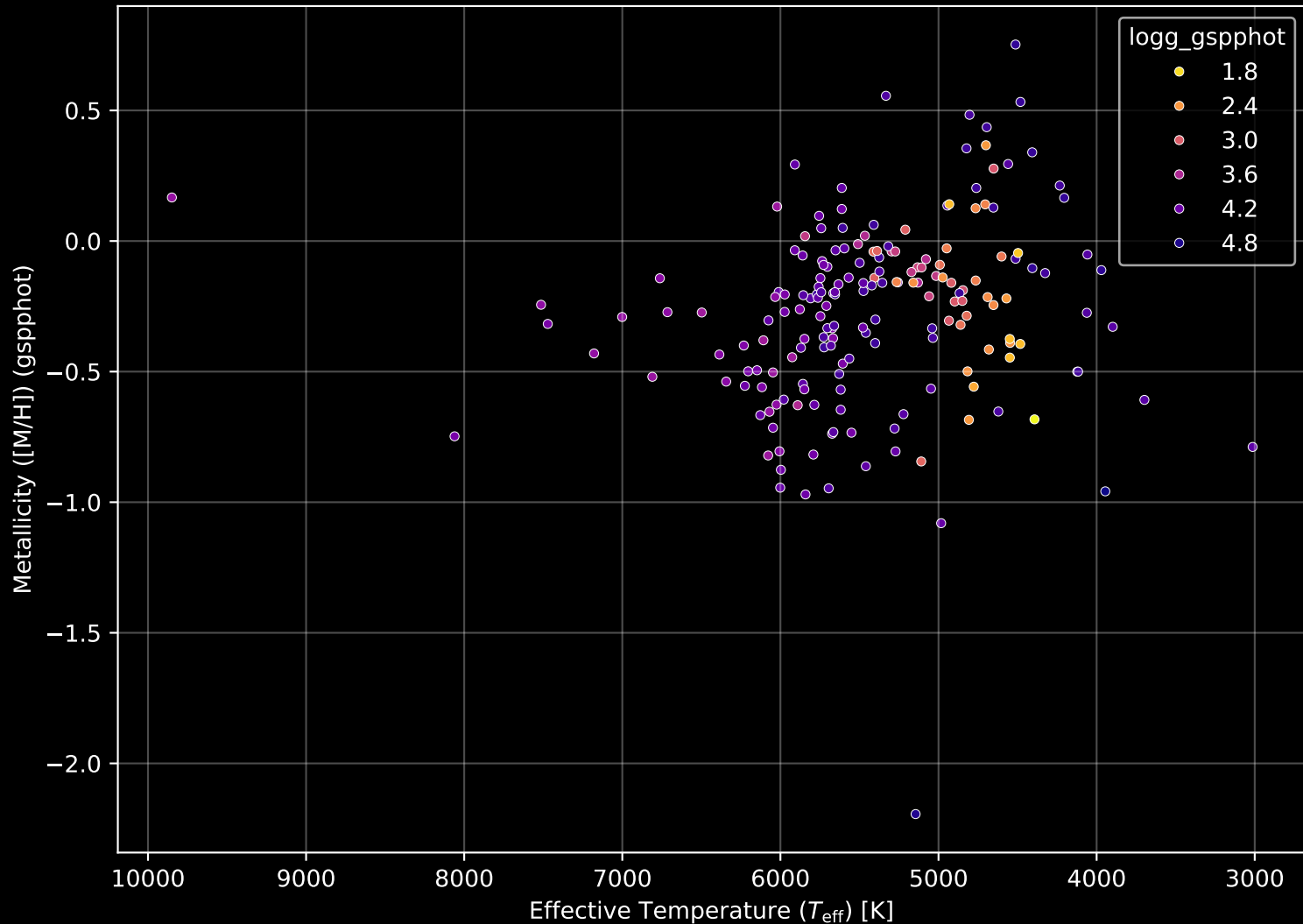
APOGEE DR17 Field: [168+30_MGA] Stellar Population Parameters (n= 186)
