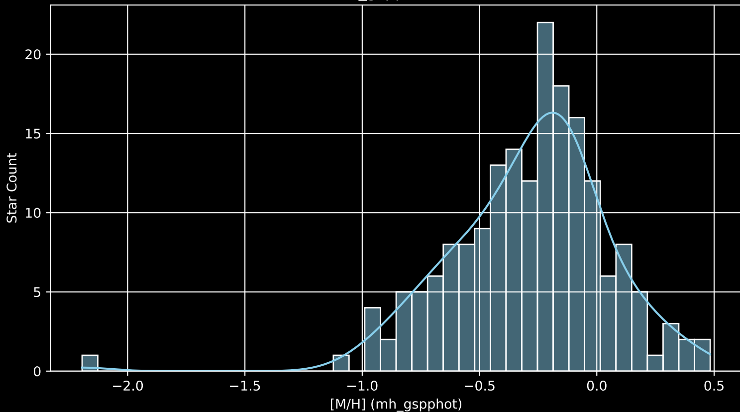
APOGEE DR17 Field: [168+30_MGA [M/H] (mh_gspphot) (n= 183)
