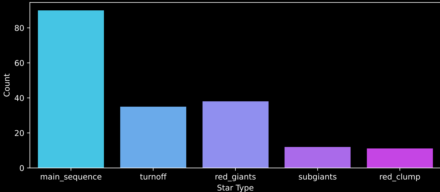
APOGEE DR17 Field: [168+30_MGA] Count plot of Star Type
