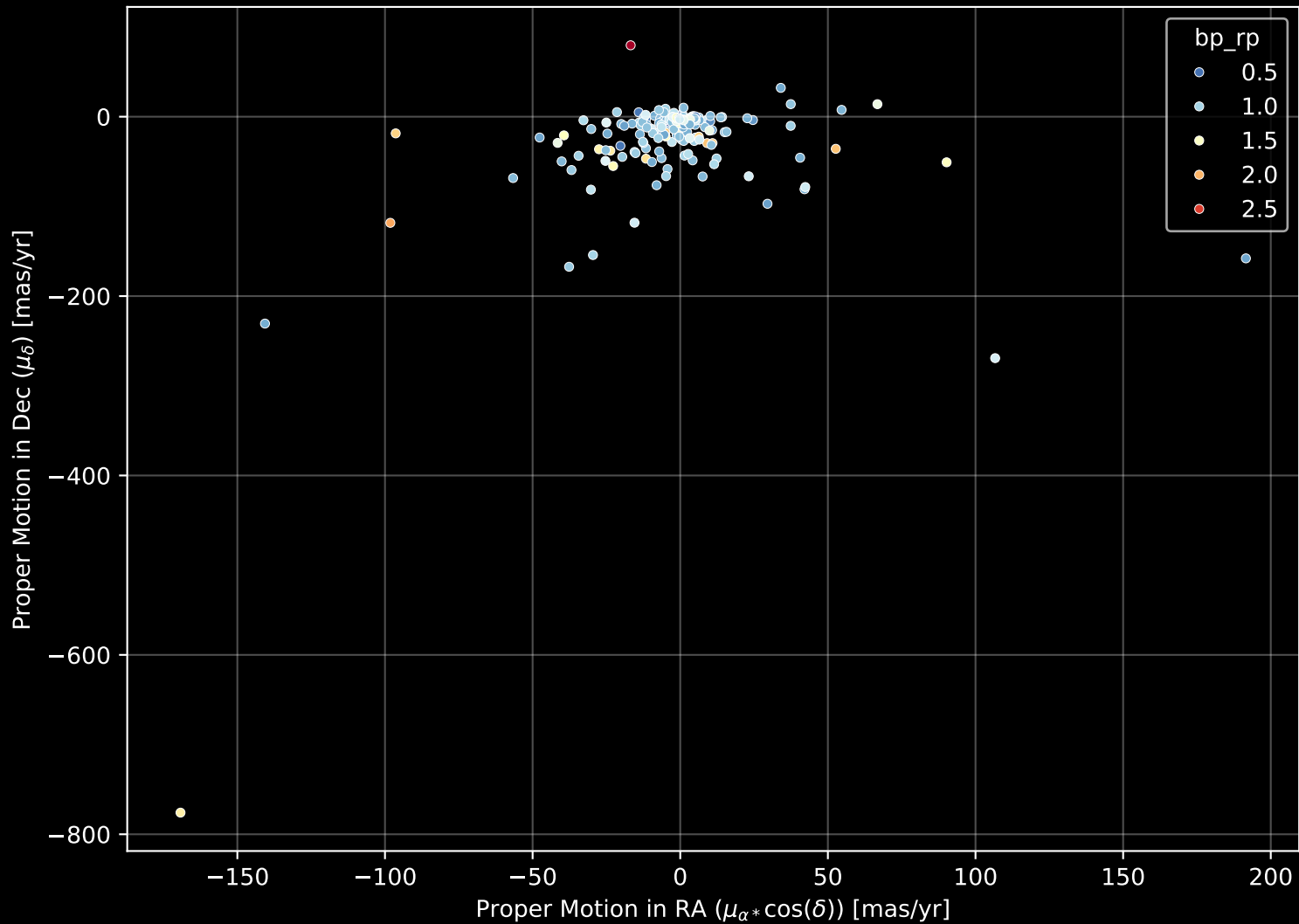
APOGEE DR17 Field: [168+30_MGA] Proper Motion Diagram (n= 186)
