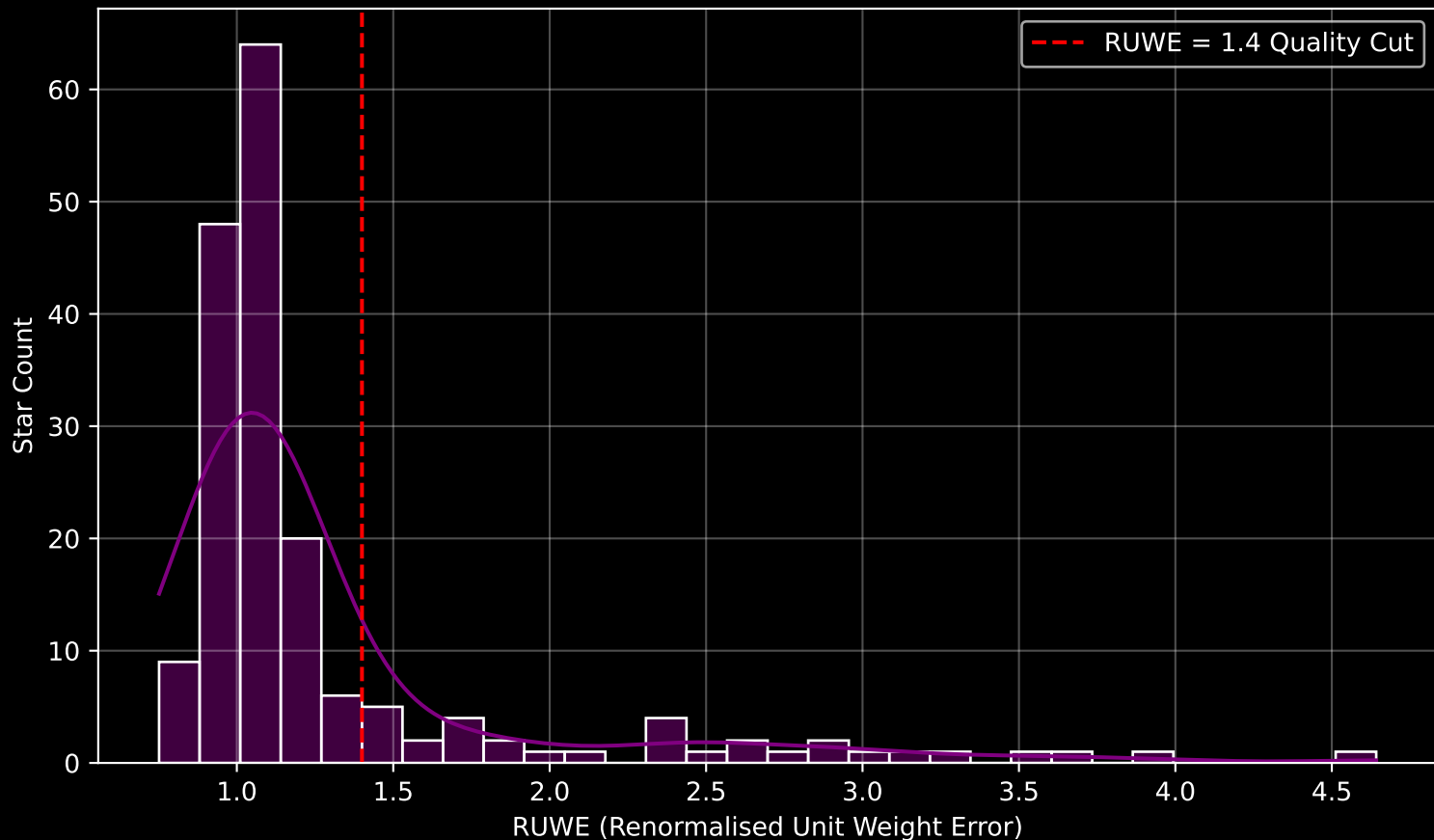
GAPOGEE DR17 Field [168+30_MGA] RUWE Distribution (n= 179)
